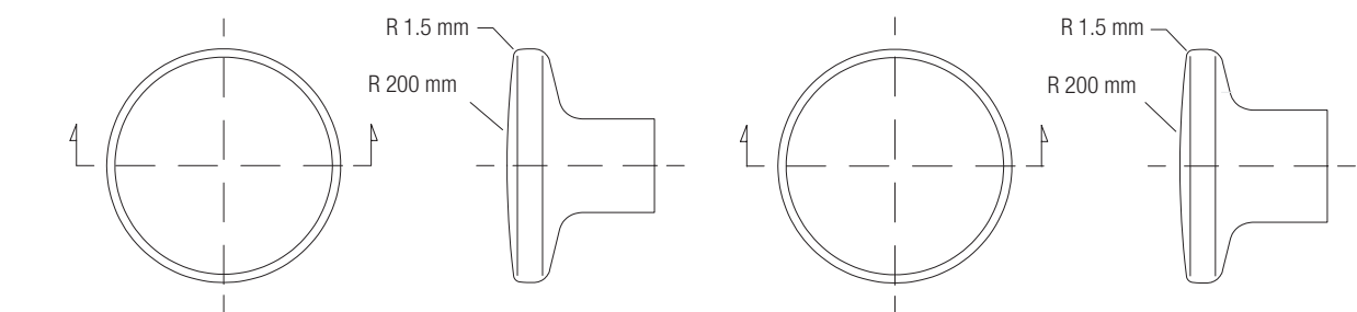
2GN - Maniglia tornita in metallo verniciato effetto ghisa. 2GN - Handle turned in varnished metal cast iron effect.
